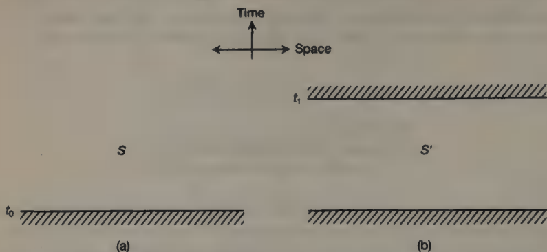
Figure 3.5 Two space-times S and S' which are determined by identical sets of initial conditions prescribed on the surface of initial time t_0 . In the case (a), the space-time S is maximally extended, whereas in (b) it is brought to an end arbitrarily at some future time t_1 , but no physical infinity or other defect in the space-time structure arises then; the space-time S' is therefore identical to S up to the time t_1 , but does not exist to the future of that moment. In practice, it is always assumed that a given set of initial conditions leads to the maximally extended space-time and not one of the infinite number of artificial alternatives which are identical up to some finite moment and then cease to exist for no physical reason.
