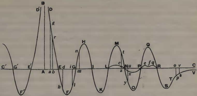
Figure 2.1 Boscovich's original universal force law, reproduced from his Theory of Natural Philosophy , first published in 1758. The variation of the force between two 'points of matter' as the distance between them changes is traced by the undulatory curve passing through the sequence of points DFHKMQSTV. The distance between them is given along the abscissa AC; the strength of the force along the ordinate AB. The force is repulsive when this curve lies above the line AC and attractive when it lies below it. At very large distances (at and beyond V), it is attractive and approaches Newton's inverse-square law of force produced by gravity. The repulsive nature of the force as the separation of the two points tends to zero prevents all matter collapsing to zero size. Regarding this picture, Boscovich remarks: 'A Law of this kind will seem at first sight to be very complicated, and to be the result of combining together several different laws in a haphazard sort of way; but it can be of the simplest kind and not complicated in the slightest degree; it can be represented for instance by a single continuous curve . . . It is sufficient merely to glance at it.'
