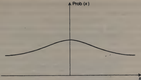
Figure 5.7 A probability distribution in which the probability is not highly peaked about any particular value. If wormhole interactions predicted that the probability of a constant of Nature, x , in our visible universe should look like this, then it is difficult to determine whether we should take the most probable value (zero here) to be the value which should correspond to reality. If a wide range of possible values of x were to give rise to universes which could neither evolve nor sustain intelligent beings, then they could not be observed. We should compare observation with the probability that the constant takes the value x conditional on that value permitting the evolution of life, and this can be a very different quantity to the unconditional probability that it take the value of x .
