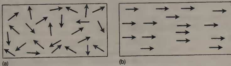
Figure 6.1 Magnetization. (a) When the temperature exceeds a critical value, the forces acting upon the atoms in a bar of metal do not distinguish any preferred directions; they are symmetrically distributed because the thermal agitations are large enough to randomize any tendency to point in preferred directions. (b) When the temperature falls below the critical level, it becomes energetically economical for the atoms to orient themselves in the same direction; any direction could be randomly chosen, but, after it has been, the directional symmetry of (a) is broken and North and South Poles are established in the bar magnet.
