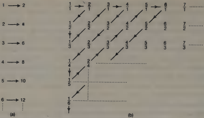
Figure 3.1 (a) The positive even numbers form an infinite set of the same 'size' as all the positive integers because the two sets can be put into the direct one-on-one relationship shown here. This means that they can be systematically counted. (b) The set of all rational fractions can also be put in a one-on-one relationship with the positive integers and hence be systematically counted if they are listed in the pattern shown and then counted in the order marked by the sequence of arrows, ad infinitum .
