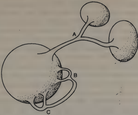
Figure 5.5 Some conceivable interconnections involving wormholes and baby universes not permitted by the 'dilute wormhole' approximation which is required to make the calculations of the wormhole-induced constants of Nature tractable at present. At A, B, and C see wormholes dividing, whilst at B and C we see wormholes that do not join large flat regions. By contrast, the configurations shown in Figures 5.2 and 5.3 were completely in accord with the dilute wormhole approximation.
