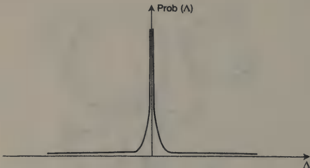
Figure 5.4 The probability that, when measured in a low-energy world like our own, the cosmological constant will be found to possess a value \Lambda is a result of wormhole interactions to neighbouring baby universes. It is very steeply peaked about zero.
