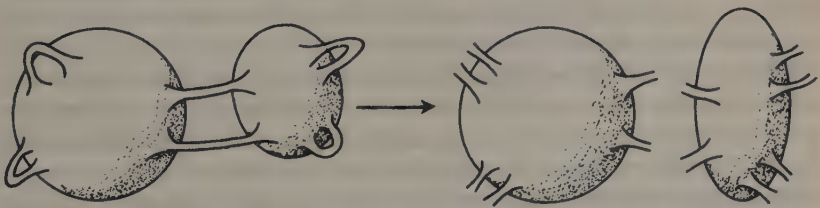
Figure 5.6 In the dilute wormhole approximation, the effects of the wormhole connections can be represented as the effects of the connected pieces that result after the wormhole connections are cut.
