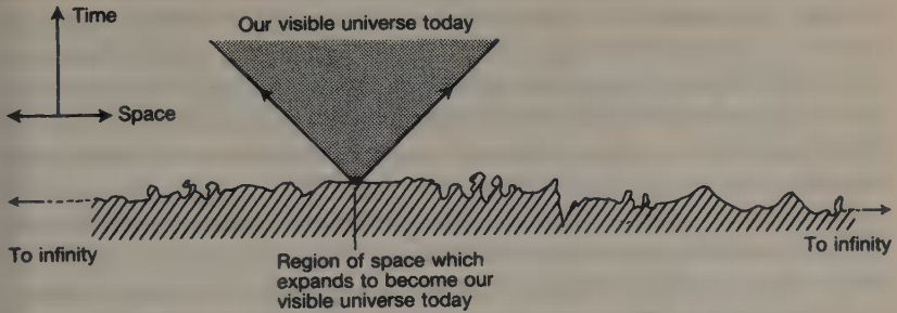
Figure 3.3 The structure of the visible universe is determined by conditions over only a tiny part of the 'initial' conditions of the Universe. If the Universe is infinite in size, then both our visible part of it and the part of the initial conditions which determine it are but infinitesimal parts of the whole.
