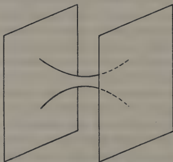
Figure 5.2 A wormhole joining two flat regions of space-time undistorted by the presence of mass-energy.
