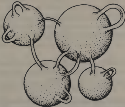
Figure 5.3 Wormholes connecting different 'universes' to themselves by handles and to other universes by wormhole 'throats'.
